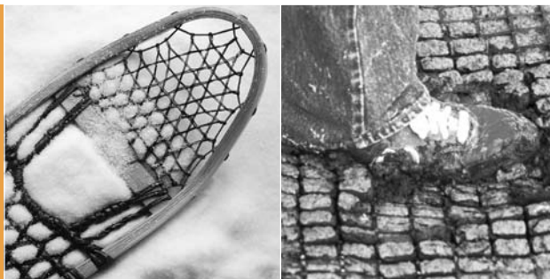
Figure 1: The Snowshoe Effect – Tensar BX Geogrids distribute heavy loads over soft soils just like a snowshoe supports the weight of a man over soft snow.
