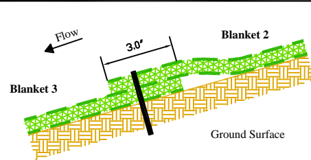
Figure B - Profile View
