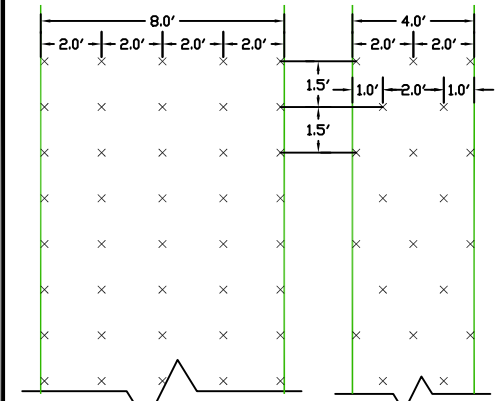
Figure D - Plan View
