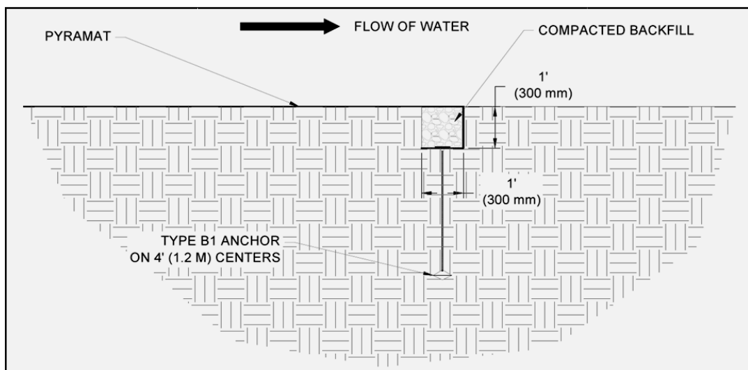
Figure 1: Initial Channel (IC) Trench
