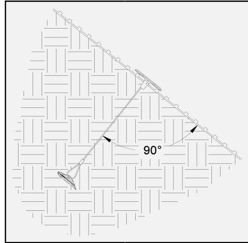
Figure 12: Complete Type B1 Anchor Installation
