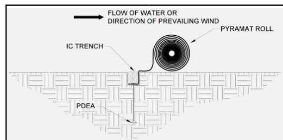
Figure 14: Initial Channel (IC) Trench Placement
