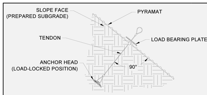
Figure 4: Type B1 Anchor Detail
