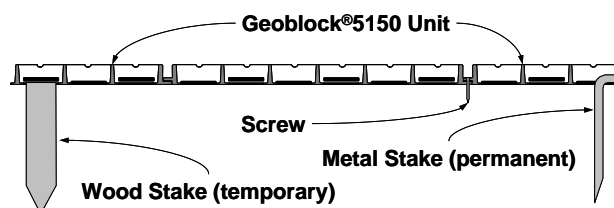
Figure 9 Anchoring Possibilities
