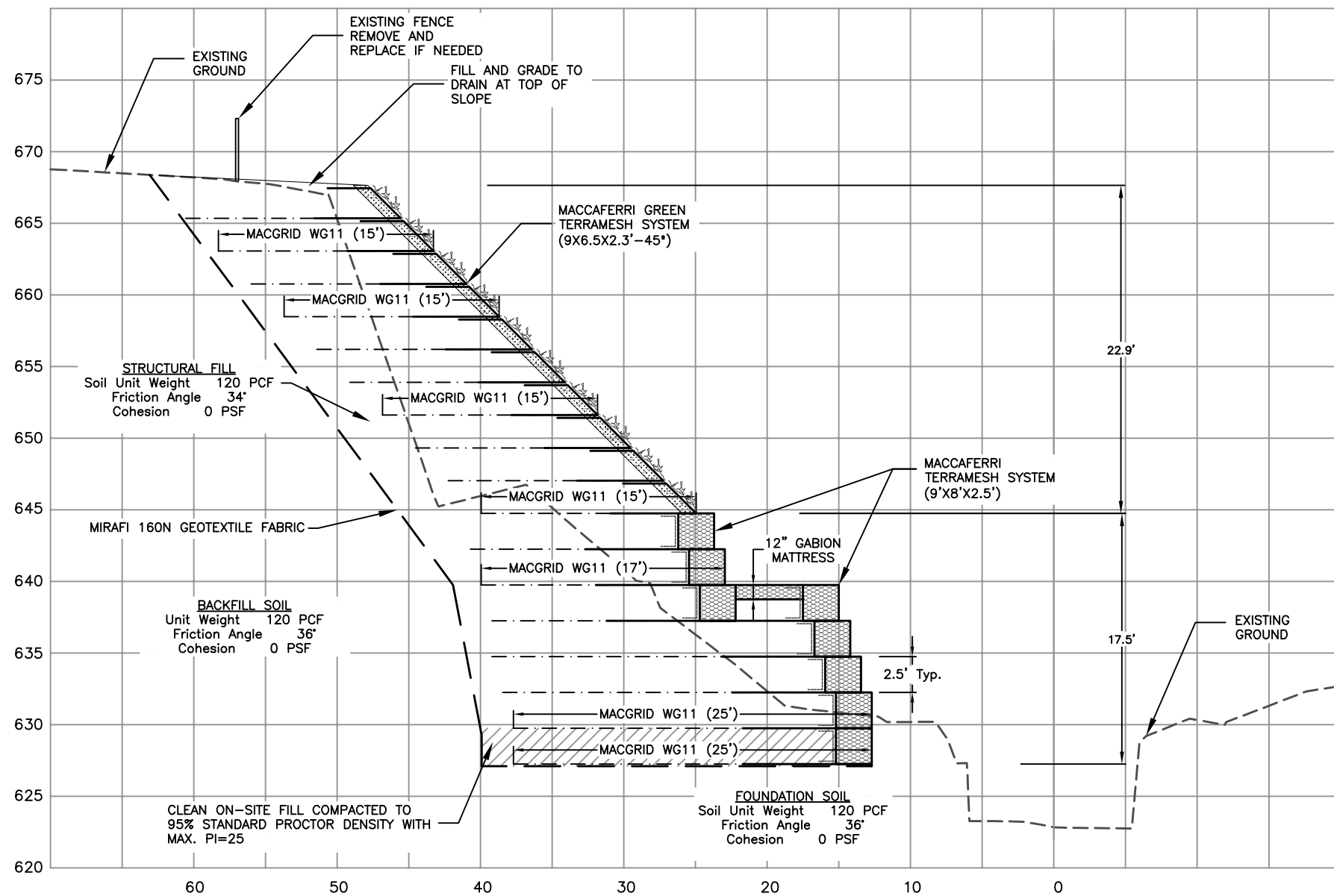
CROSS SECTION @ STA. 10+00.01 Maccaferri MSE System
