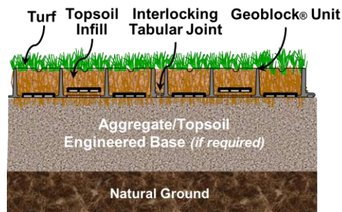
Figure 1 The Geoblock5150 Porous Pavement System Components
